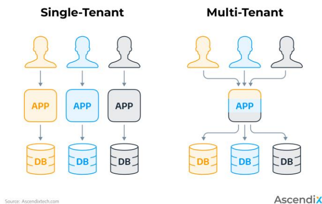
Figure 8: Single-Tenant vs Multi-Tenant [27]
