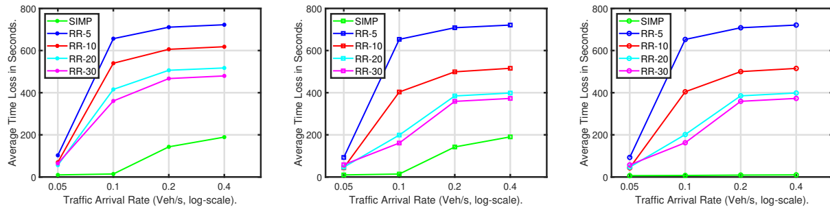
Fig. 4: Average Time Loss results in seconds, for Scenarios-1, 2, and 3 with 50\text{Km/h} speed limit from left to right.
