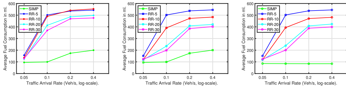
Fig. 5: Average Fuel Consumption results in \text{ml} , for Scenarios-1, 2, and 3 with 50\text{Km/h} speed limit from left to right accordingly.
