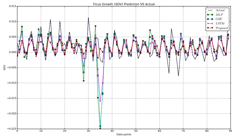
Figure 6: Obtained accuracy in two-step prediction of Ficus growth (SVD) by the proposed and baseline methods
