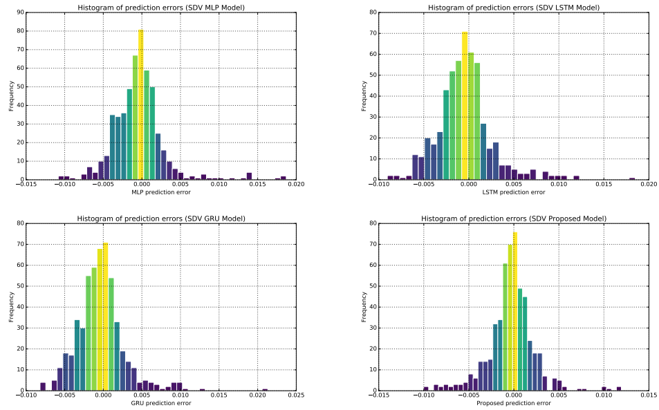
Figure 5: Error distribution for one step prediction (1 hour ahead)
