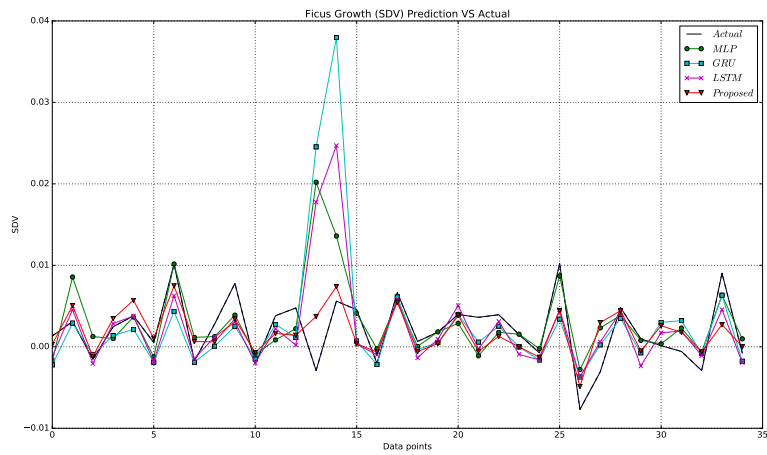
Figure 8: Obtained accuracy in three-step prediction of Ficus growth (SVD) by the proposed and baseline methods
