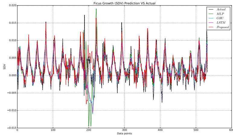
Figure 4: Obtained accuracy in one-step prediction of Ficus growth (SVD) by the proposed and baseline methods
