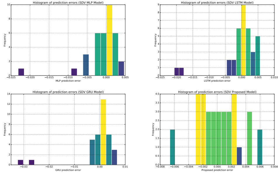
Figure 9: Error distribution for three step prediction (12 hour ahead)
