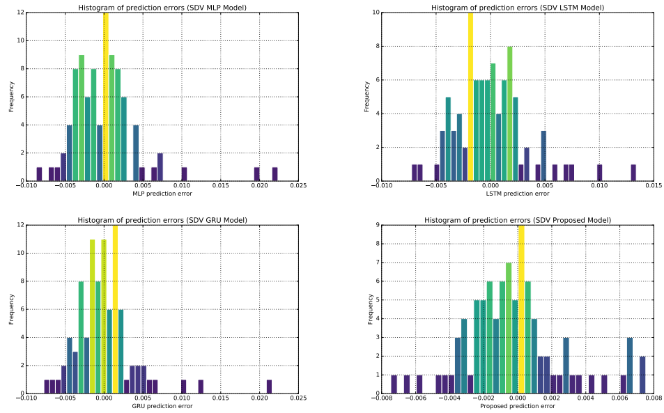
Figure 7: Error distribution for two step prediction (6 hours ahead)
