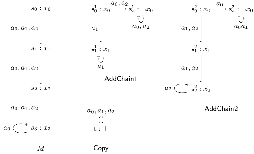
Fig. 5. Model M , and action models AddChain1, AddChain2, and Copy.
