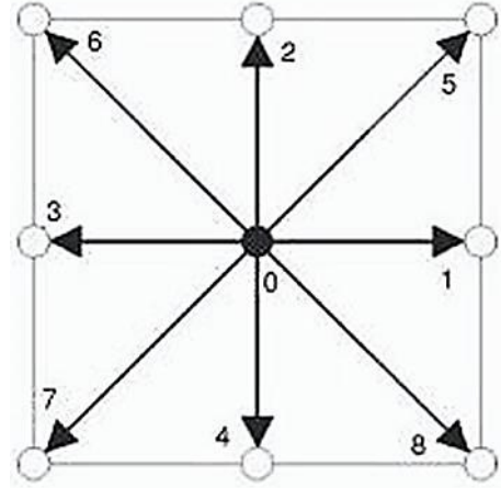
Figure 4. D2Q9 Lattice model
