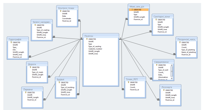
Fig. 1. Database schema view
