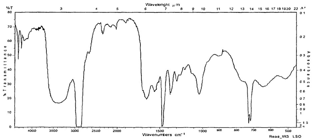
Fig. 4. IR spectroscopy of ACF and UFR resins mixture
