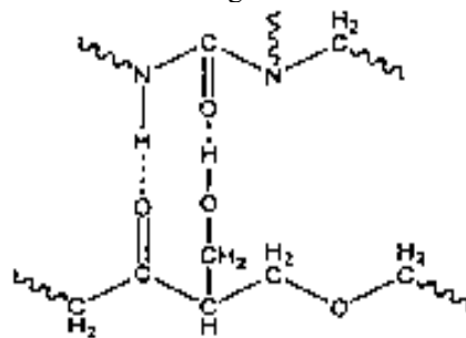
Fig. 1. The structure of the interpolymer UACF complex
